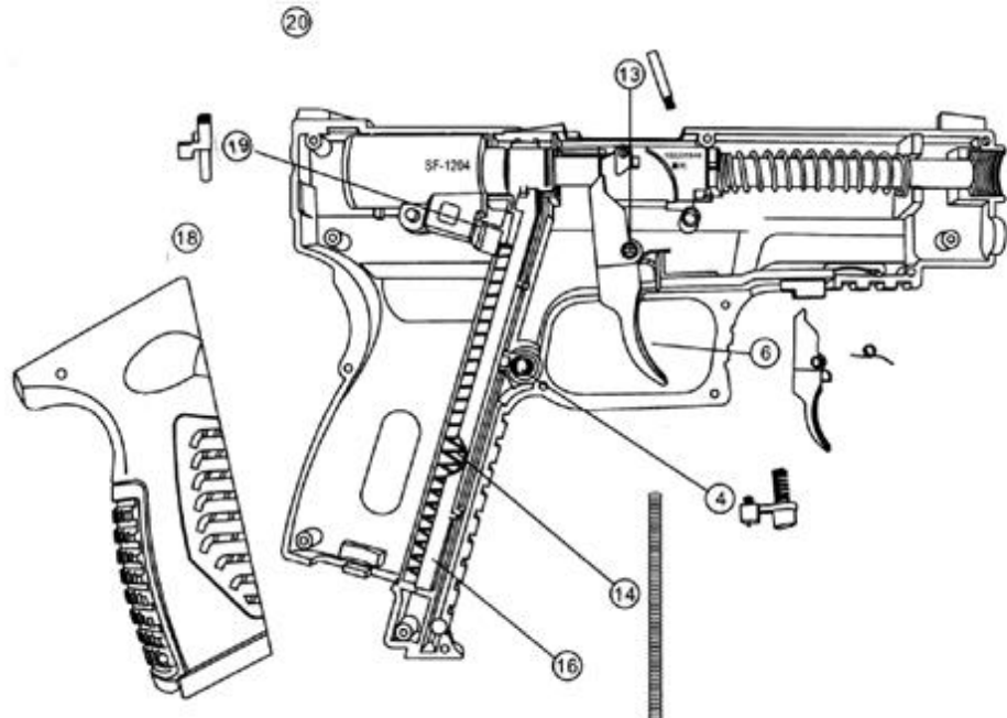
EXPLODED VIEW
